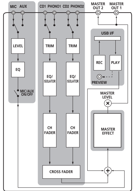
Stroomschema audiosignalen
